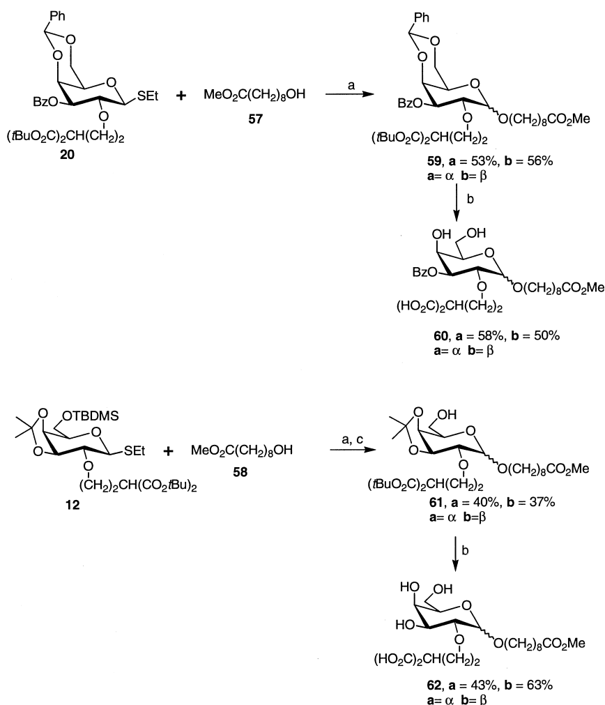
Scheme 5. (a) DMTST, 2,6-di- t Bu-4-Me-pyridine, solvent, mol. sieves; (b) TFA 90%, anisole; (c) n Bu 4 NF, THF, AcOH.
