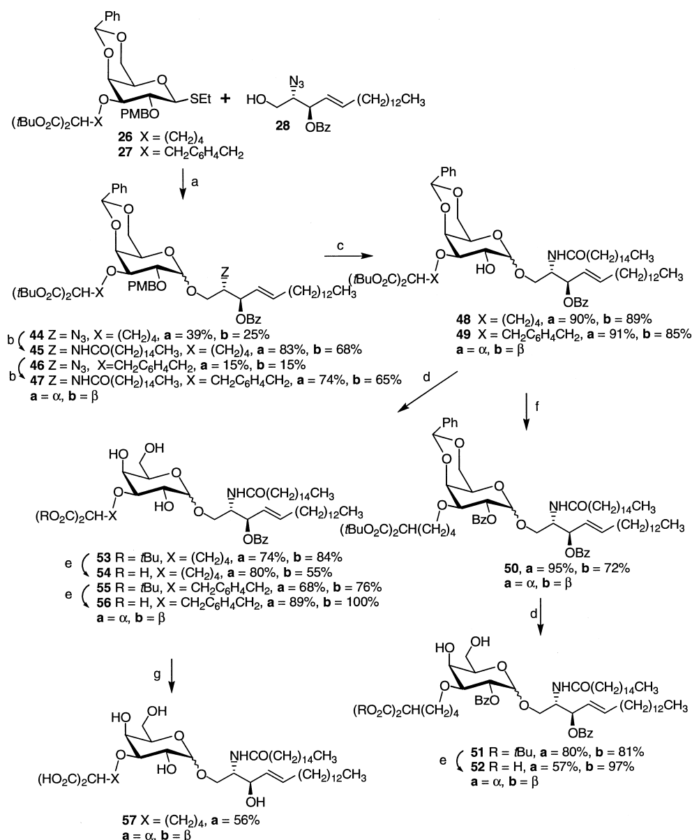
Scheme 4. (a) DMTST, 2,6-di- t Bu-4-Me-pyridine, solvent, mol. sieves; (b) (1). H_2S , pyridine, H_2O ; (2) CH_3(CH_2)_{14}COCl , NaOAc , THF; (c) DDQ, CH_2Cl_2 , H_2O ; (d) TFA 90%, CH_2Cl_2 , (e) TFA 90%; (f) BzCl , pyridine, DMAP; (g) MeONa .
